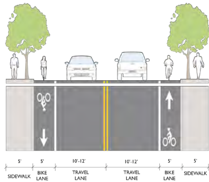
BIKE LANE + SIDEWALK
