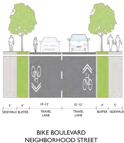
Figure B-7: Neighborhood Bikeway Cross Section
